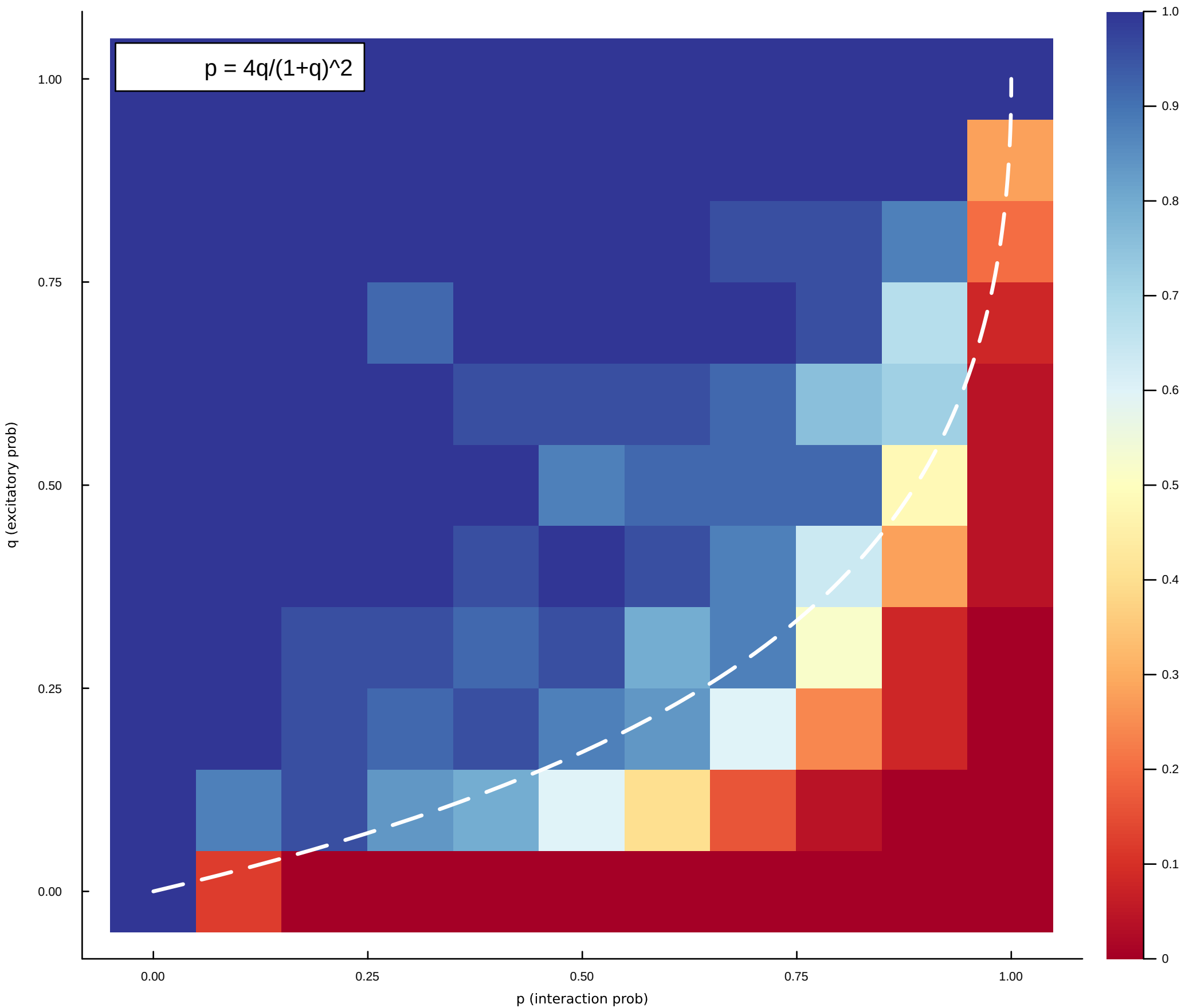
Convergence Heatmap (N=100)
